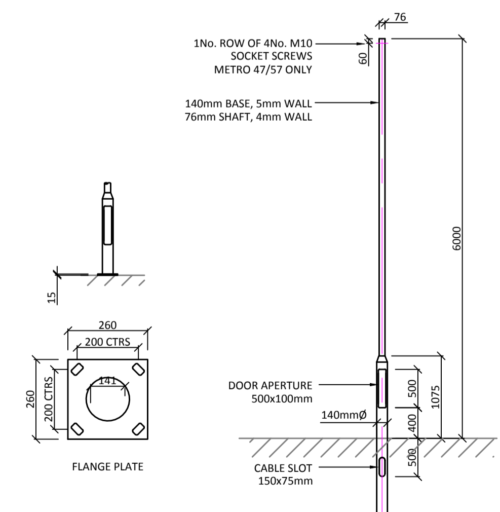
DETAIL No.1 TYPICAL 6 METRE POLE LIGHTING COLUMN SCALE N.T.S.
